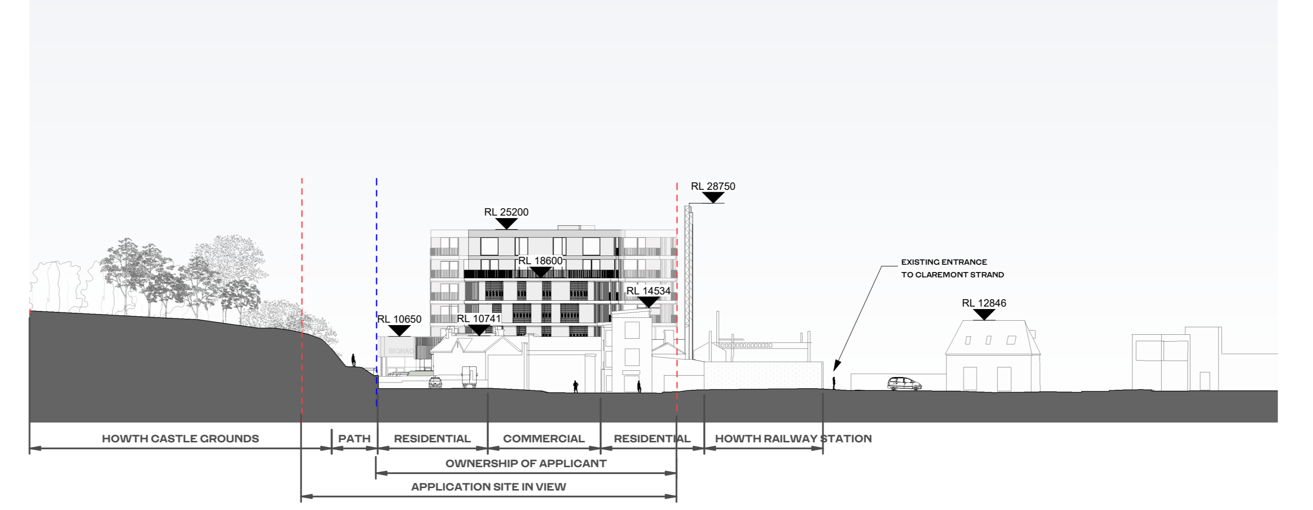
4 CONTIGUOUS ELEVATION - EAST 1:500
