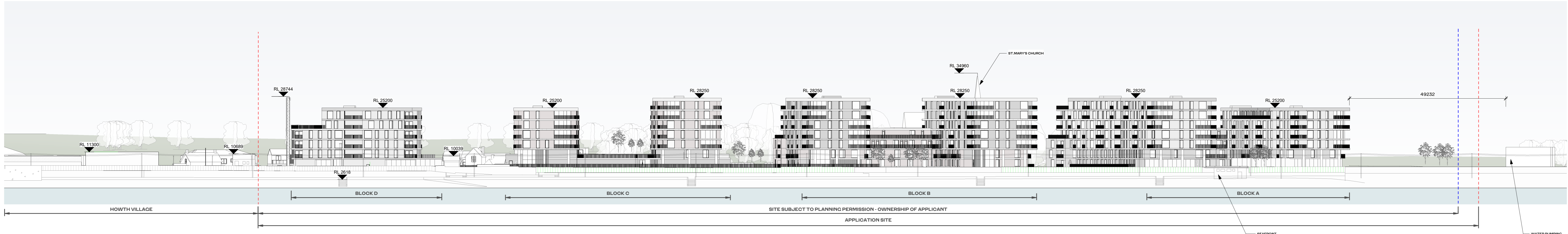
1 CONTIGUOUS ELEVATION - NORTH 1:500
